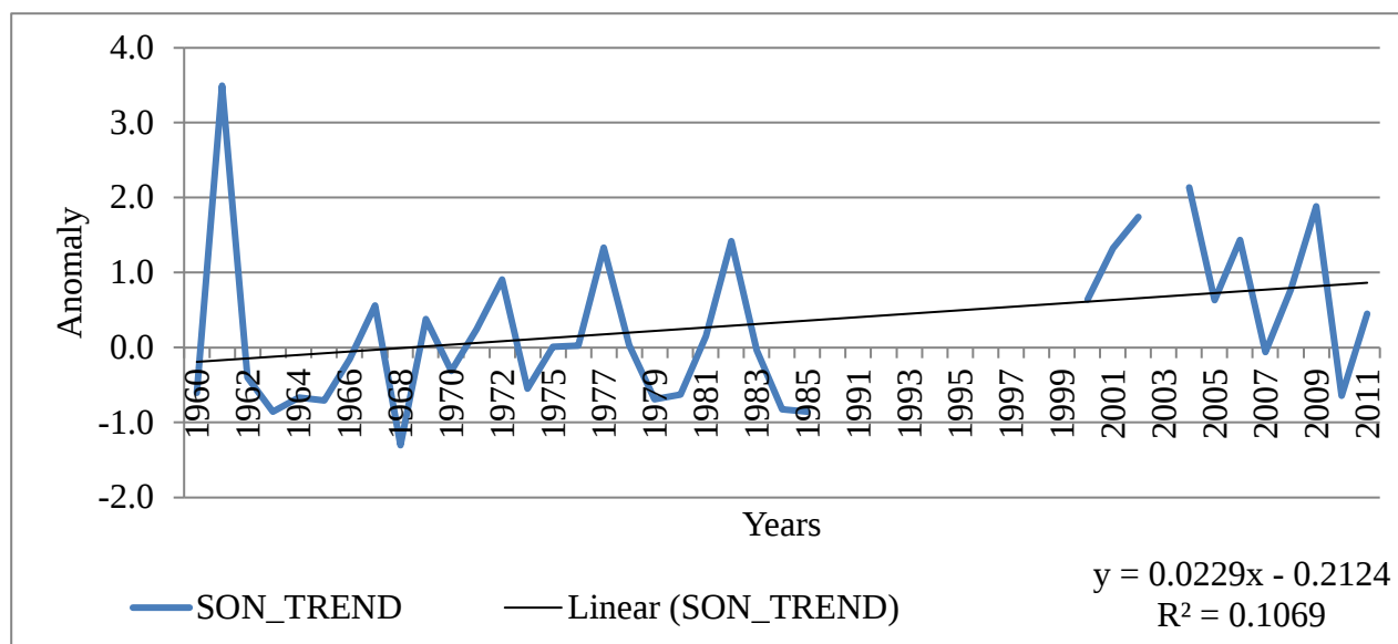
Figure 2 Karenga seasonal rainfall trend (1960 - 2011):
