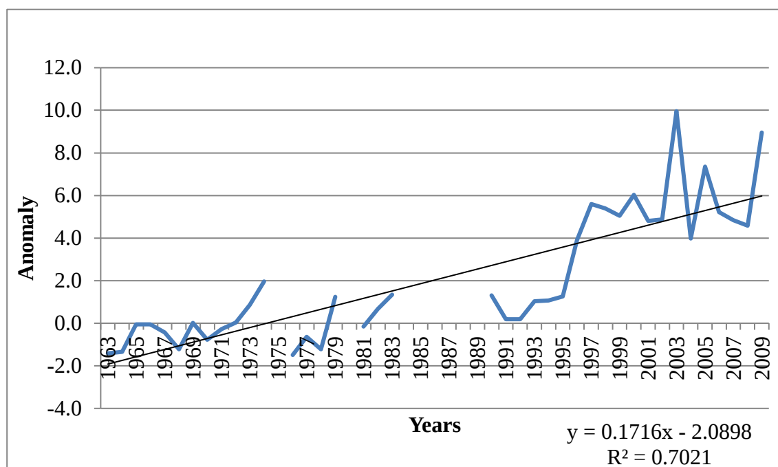
Figure 1: Karenga mean annual maximum temperature (°C) trend
