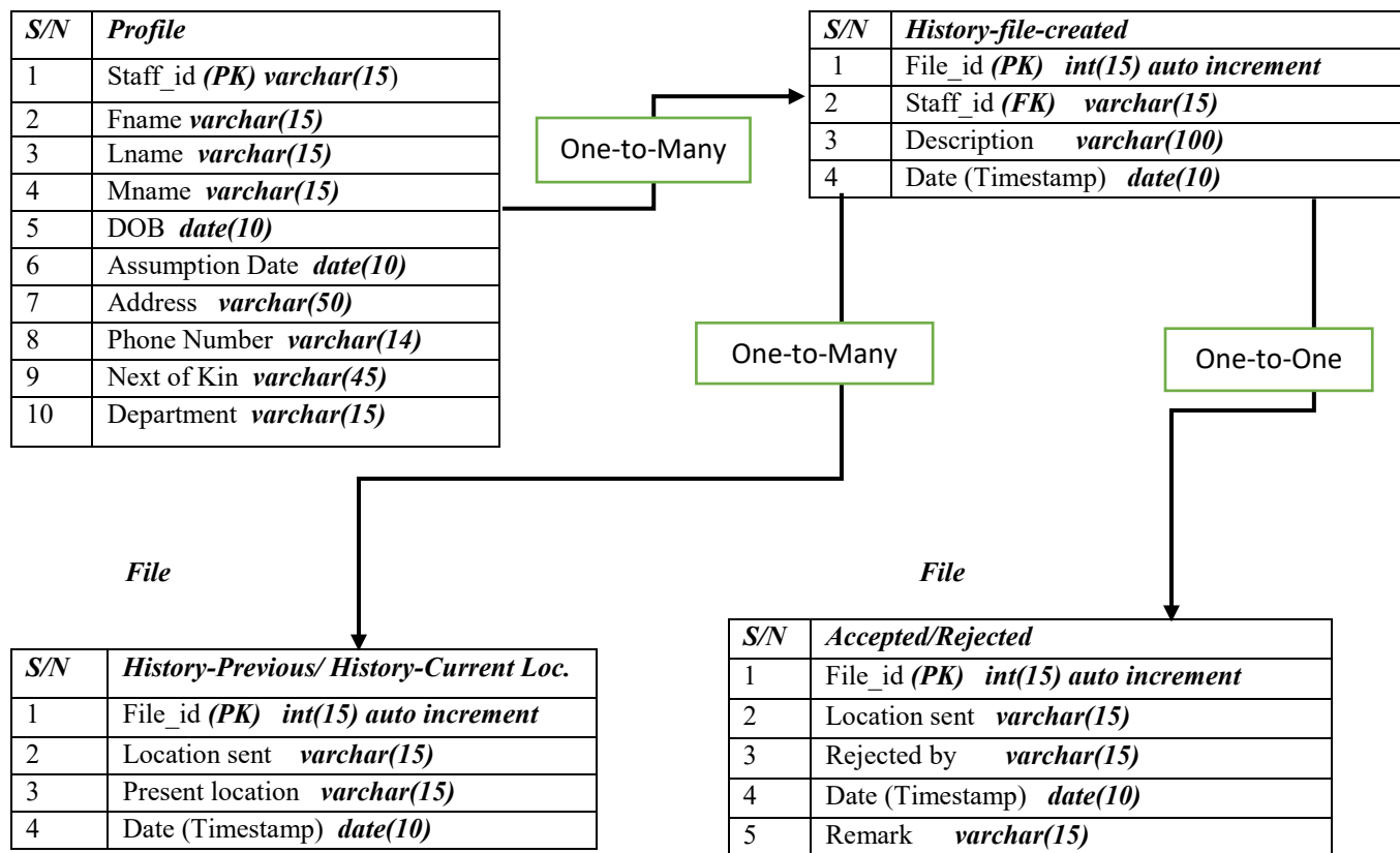
Figure 4: Database representation of Easy Design Diagram
