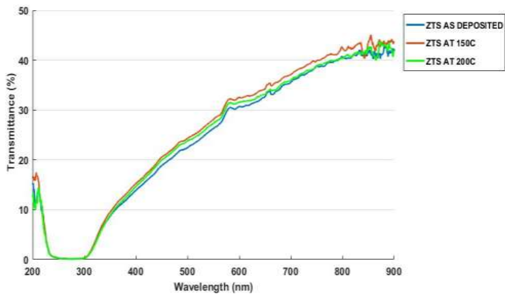
Figure 3: Graph of Transmittance against wavelength for ZTS
