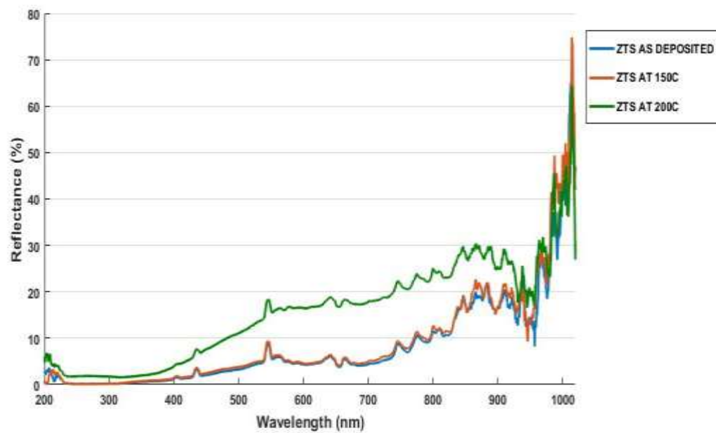
Figure 2: Graph of reflectance against wavelength for ZTS
