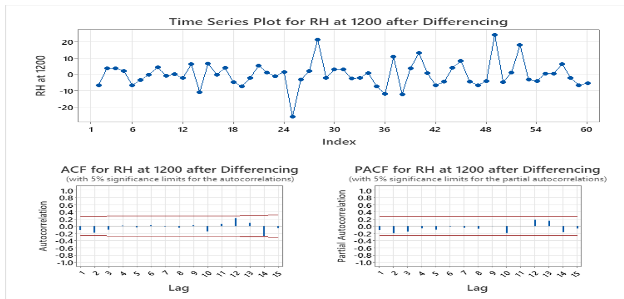
Figure 2: ACF and PACF Plots for RH at 1200 after first differencing
