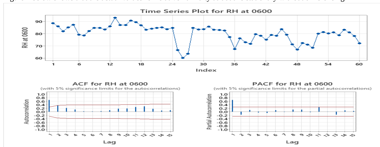
Figure 1: ACF and PACF Plots for RH at 0600
