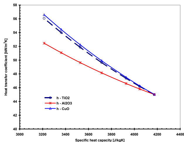
Figure 4.0 Effect of specific heat capacity on the heat transfer coefficient at 0.2 kg/s mass flow rate
