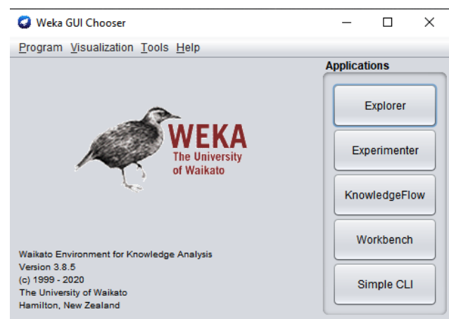
Figure 3: WEKA GUI
