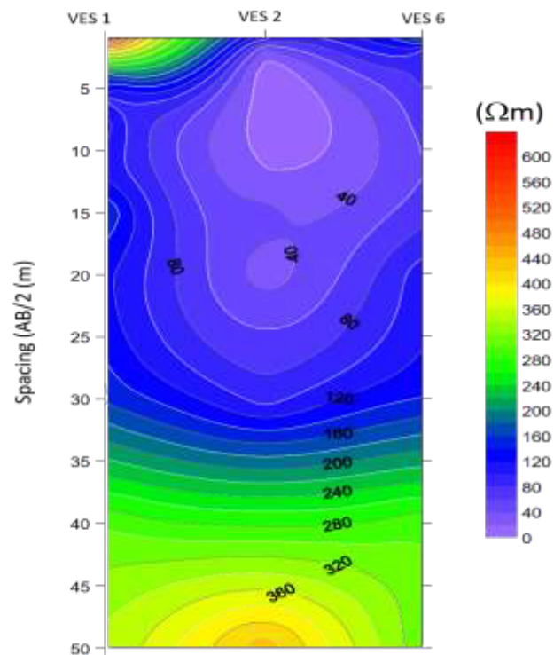
Figure 10: Pseudo-section map for profile 1
