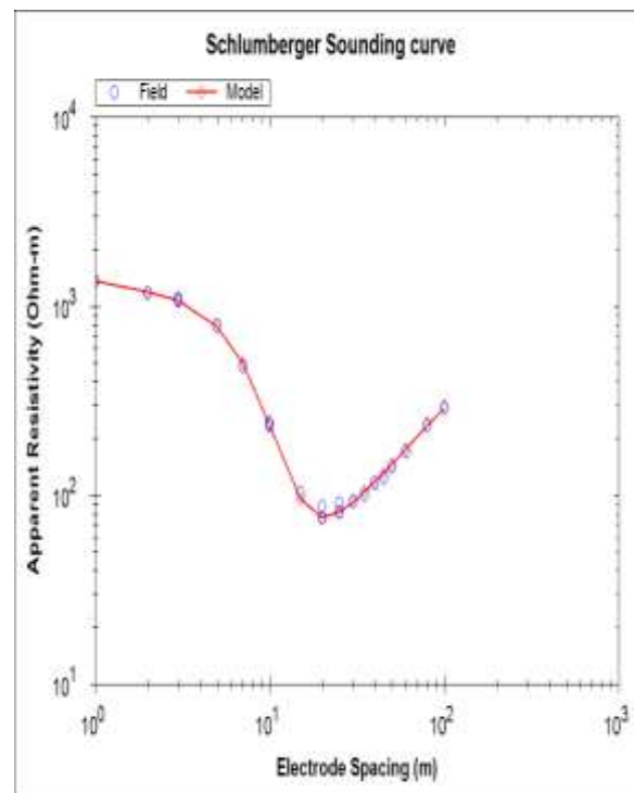
Figure 5: Resistivity plot for VES 2
