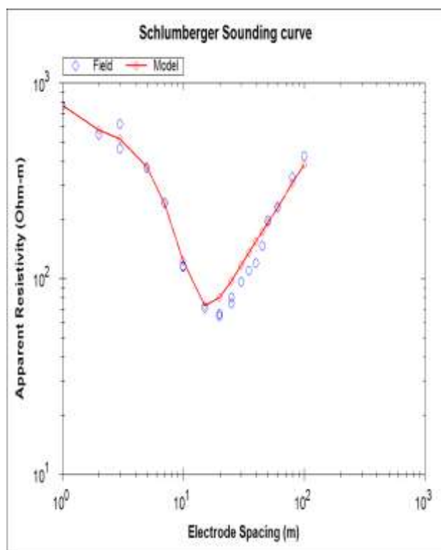
Figure 4: Resistivity plot for VES 1
