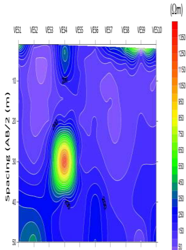
Figure 13: Pseudo-section map for the entire profile of the study area
