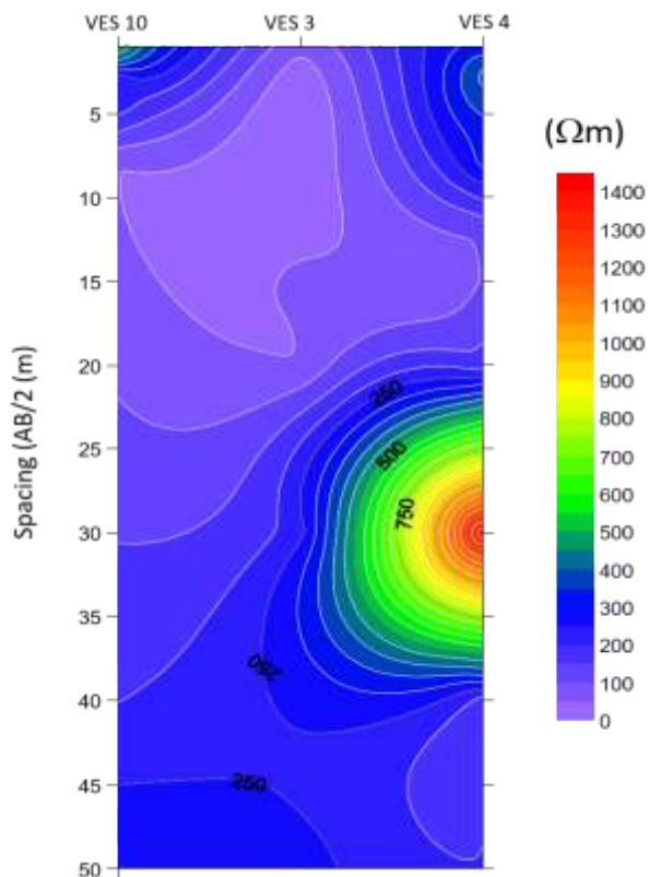
Figure 11: Pseudo-section map for profile 2
