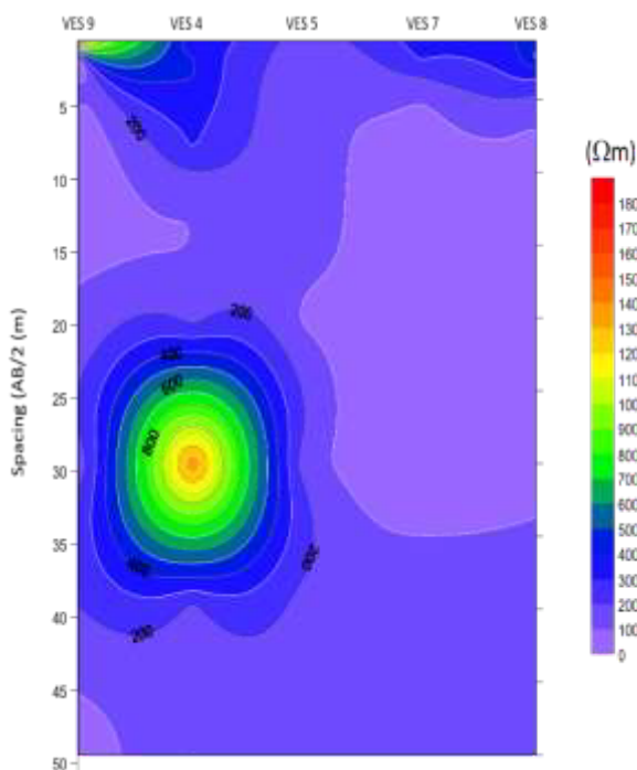
Figure 12: Pseudo-section map for profile 3
