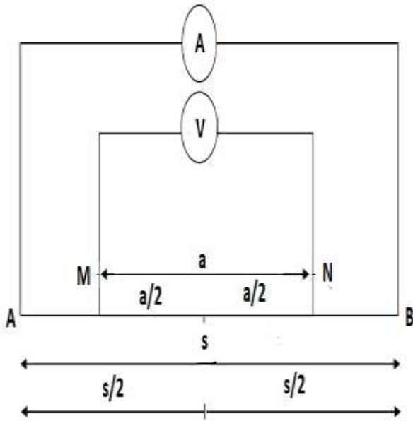
Figure 3: Schlumberger Electrode Configuration Arrangement.
