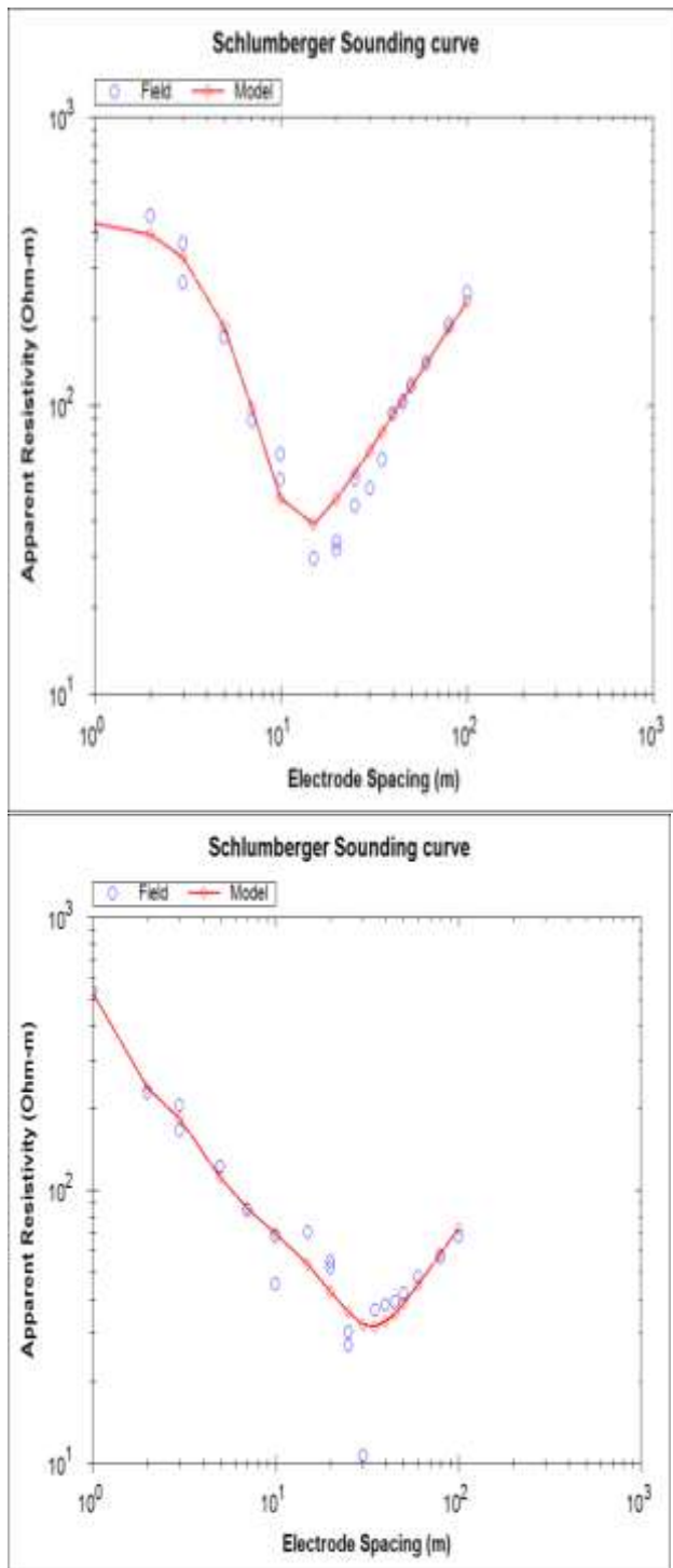
Figure 8: Resistivity plot for VES 5
