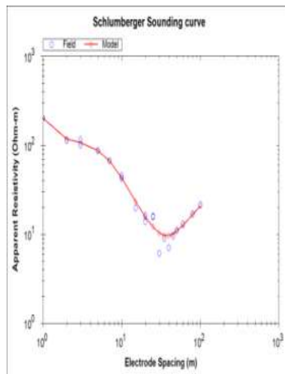
Figure 6: Resistivity plot for VES 3
