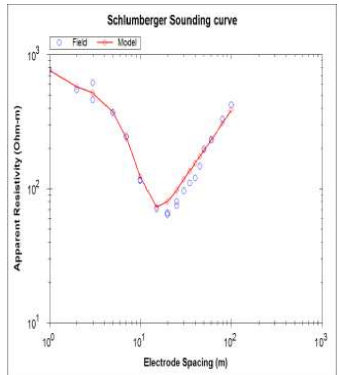
Figure 9: Resistivity plot for VES 6
