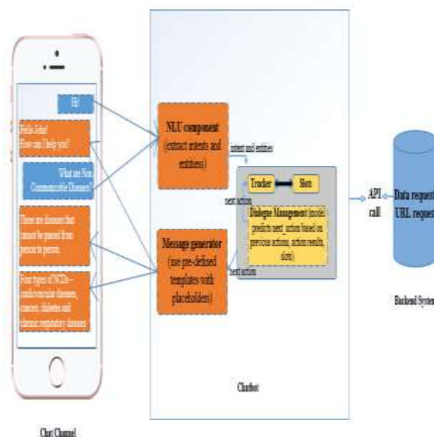
Figure 1: Chatbot Architecture. Adapted from Kompella (2018)
