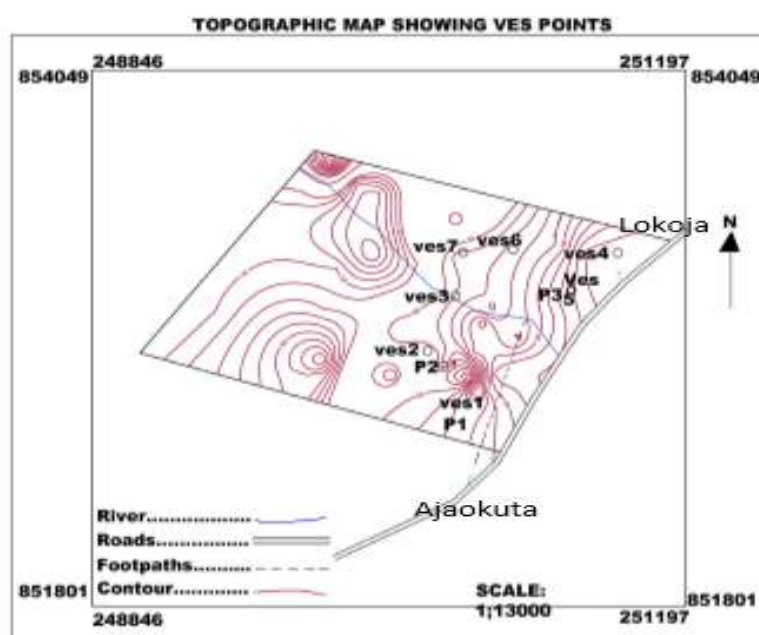
Figure 2: Topographic map of the Study Area with VES points.
