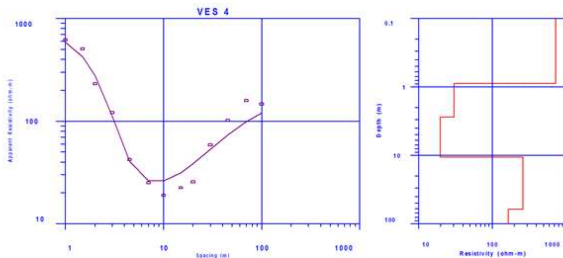
Figure 6: Resistivity curve for VES 4.
