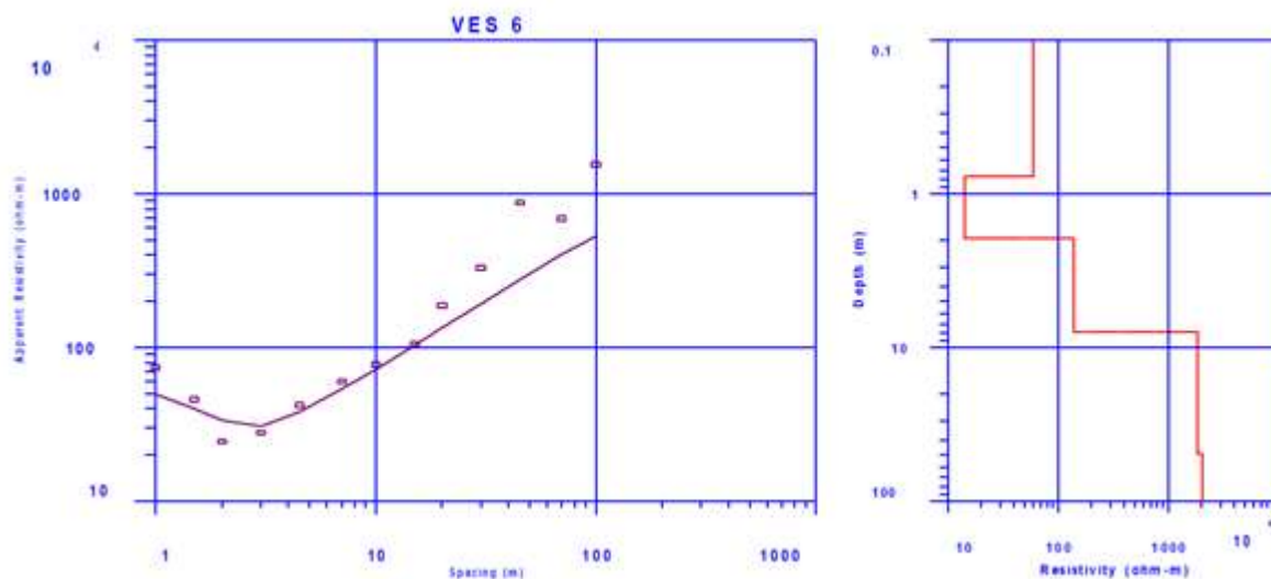
Figure 8: Resistivity curve for VES 6.
