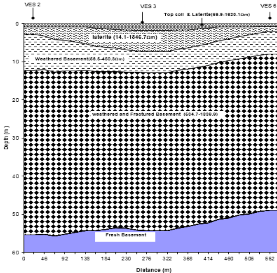
Fig 11: Geoelectric section of VES (2, 3, 6)
