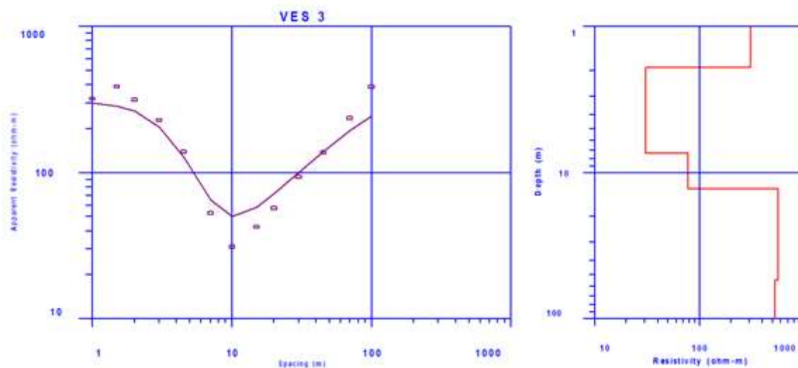
3: VES 3 LAYER MODEL
