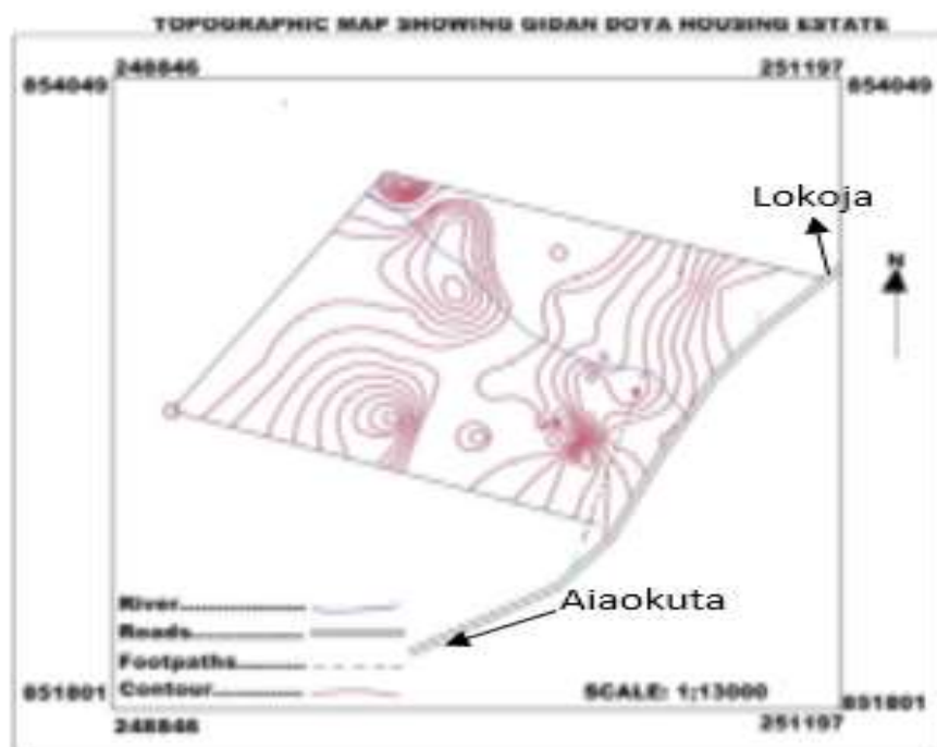
Figure 1: Topographic Map of the Study Area.
