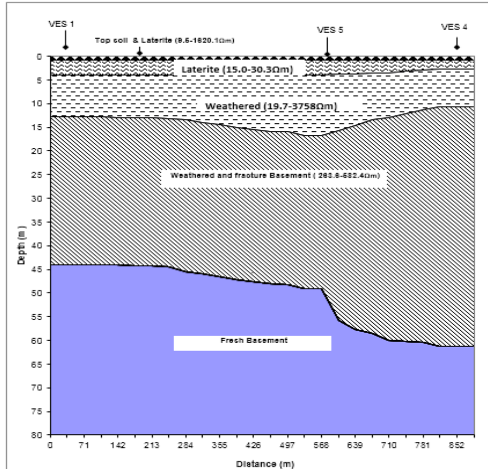
Fig 10: Goelectric section of VES (1, 4, 5)
