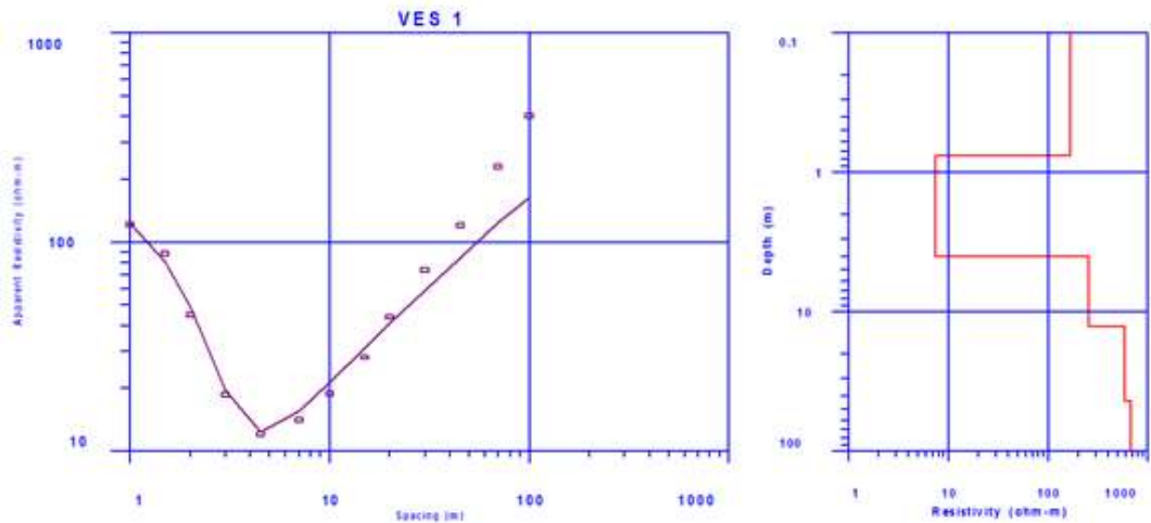
Figure 3: Resistivity curve for VES 1.
