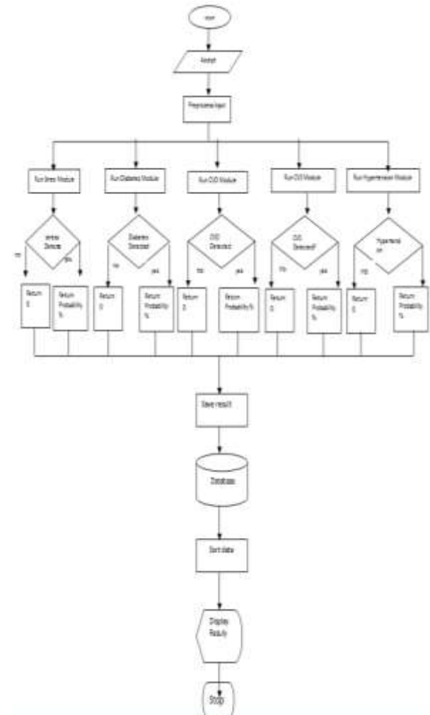
Figure 3: System Flowchart
