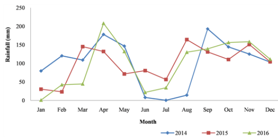
Fig 8. Comparison and enhancement of agricultural productivity
