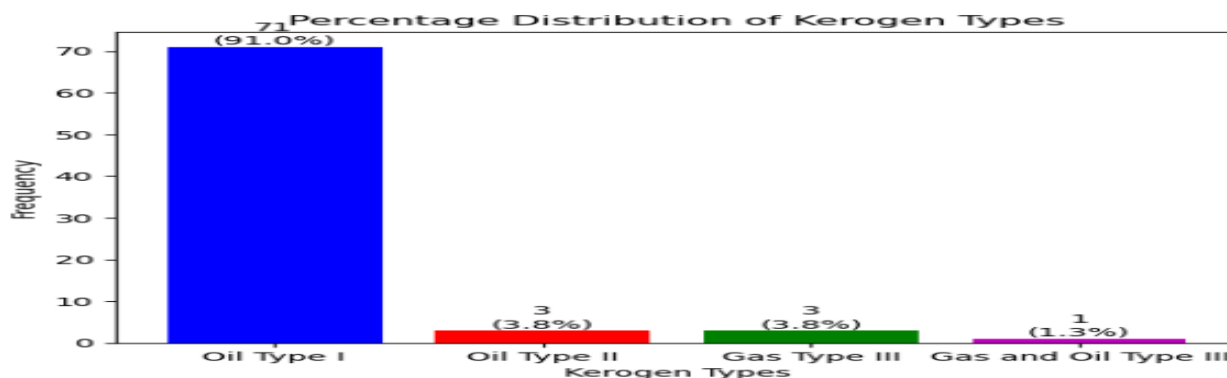
Figure 2: Bar Chart showing the Percentage Distribution of Kerogen Types
