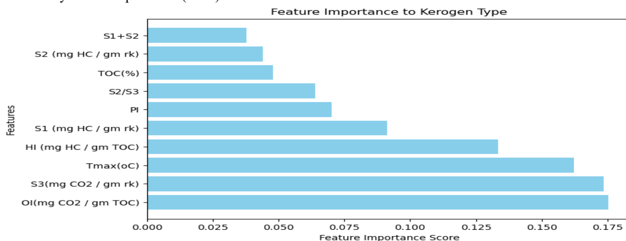
Figure 3: Bar chart showing the degree of contributions of each of the feature variables to Kerogen Types
