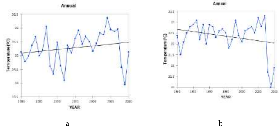
Figure 6: mean annual variation in T_{max} and T_{min} for the period 1980-2010
