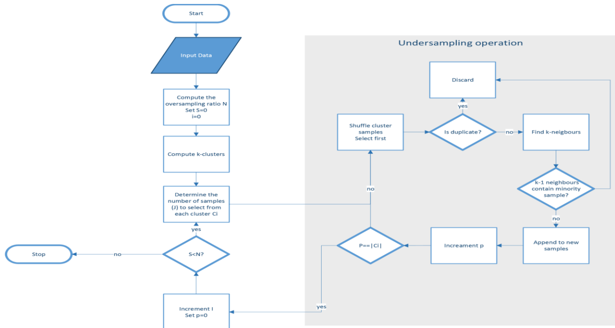
Figure 3. Under sampling Process
