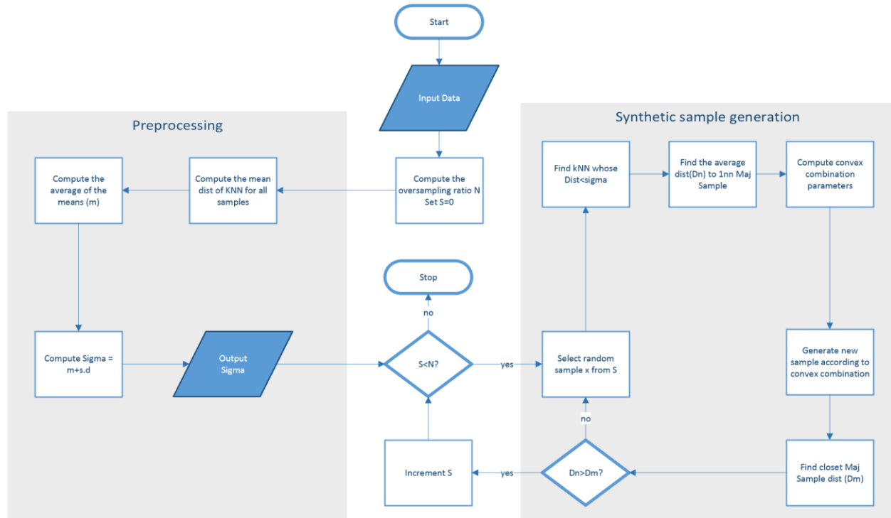
Figure 2. Oversampling Process
