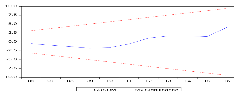
Figure 1: CUSUM
