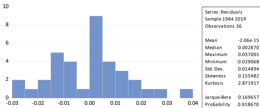
Figure 1: Normality Test
