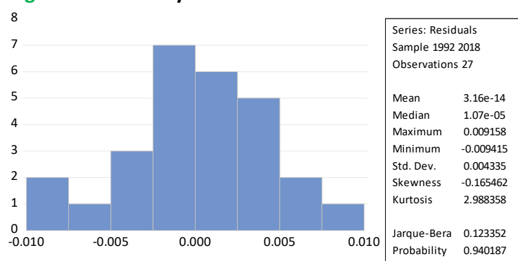
Figure 1: Normality Test
