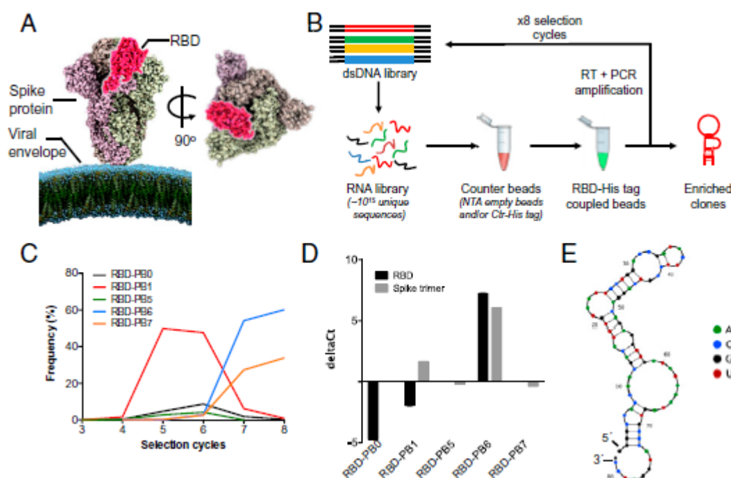
Figure 2: An RNA aptamer selection against RBD. [A] Spike protein top and side view [B] Selection scheme by SELEX [C] New Generation Sequencing data highlighting frequency (%) of the most typical RNA clones from the SELEX process. (D) The binding assay (qPCR) of five selected clones to RBD [E] RBD-PB6 secondary structure
