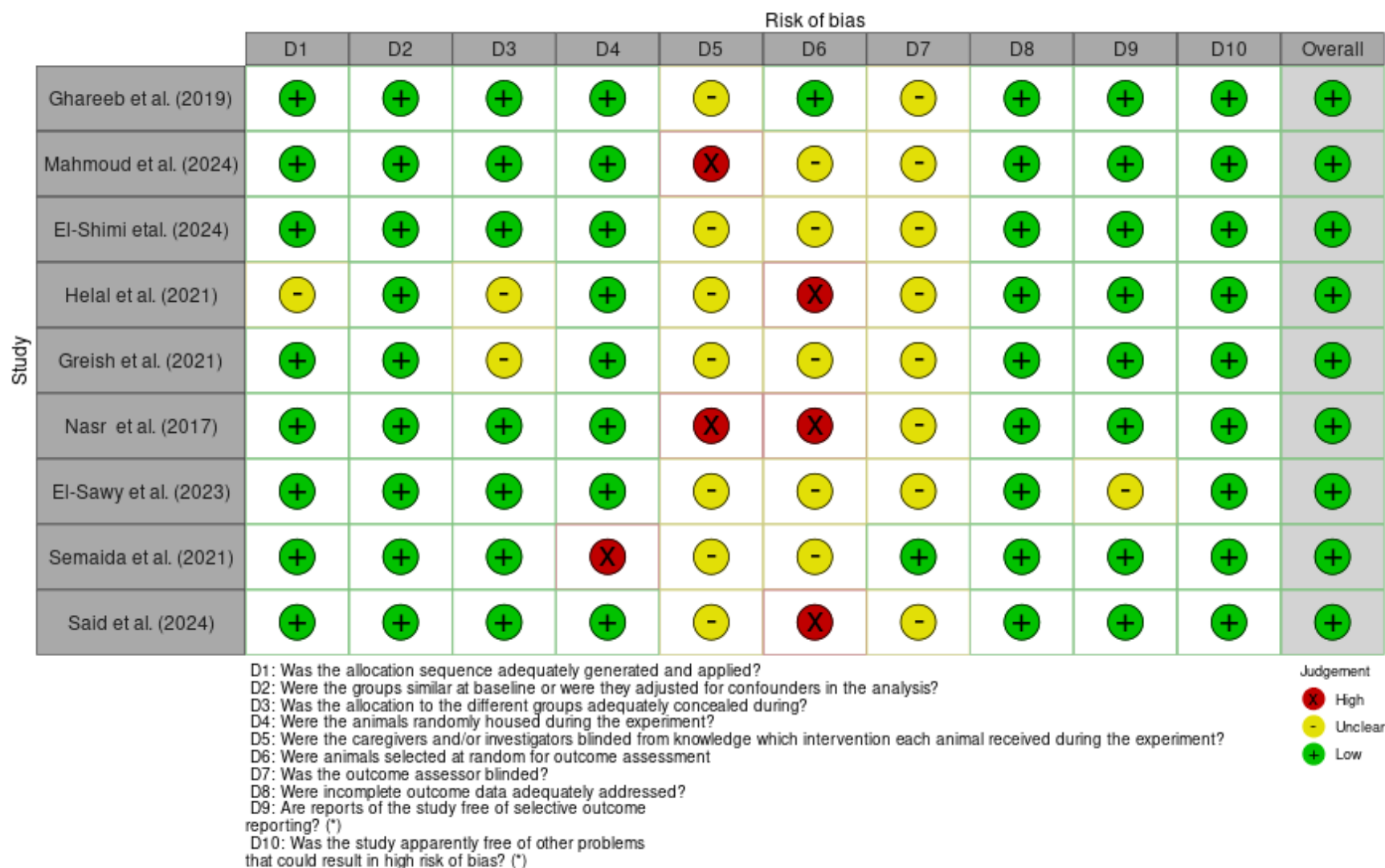
Figure 3: Bias Risk for Individual Articles
