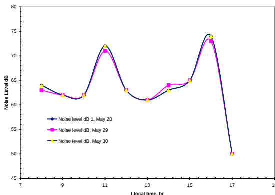
Fig. 9.0 Plot of Noise level, dB against Local Time at Different Days
