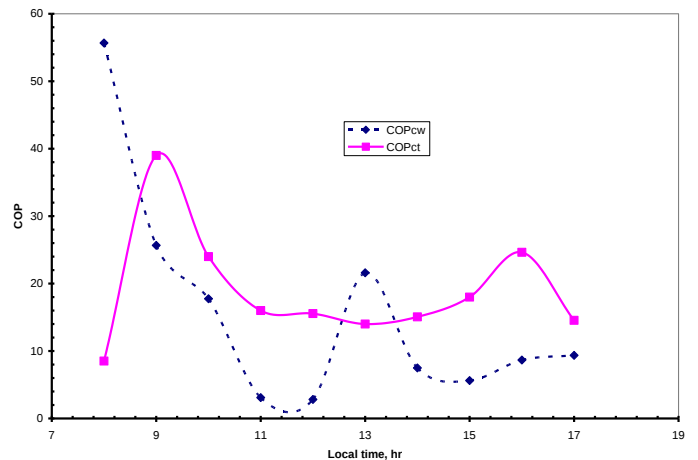
Fig. 7.0 Plot of COP of Cooling Water Tower And Cooling Water against Local Time
