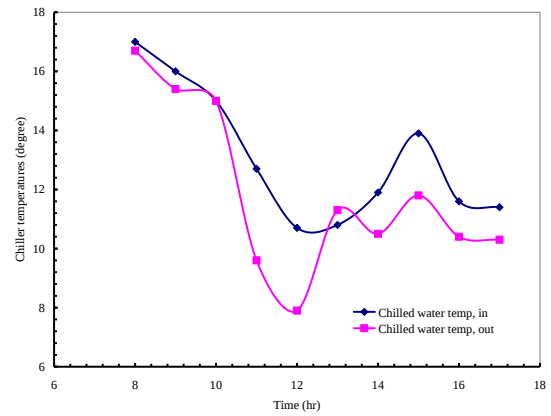
Fig. 10 Plot of Chiller Water Inlet And Outlet Temperatures against Local Time
