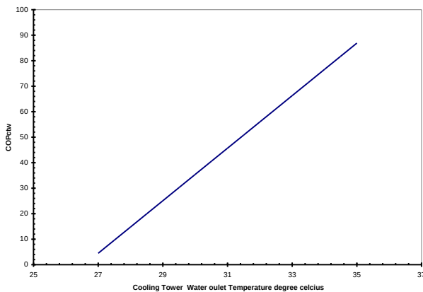
Fig. 5.0 Plot of COP of Cooling Tower against Outlet Cooling Tower Temperature
