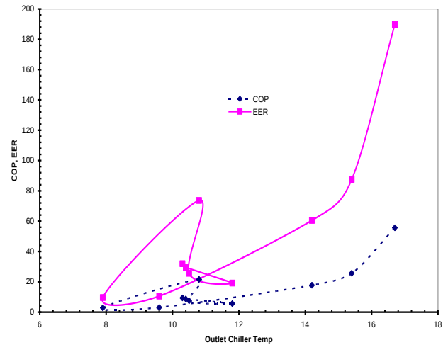
Fig. 2.0 Plot of COP and EER against Outlet Chiller Temperature
