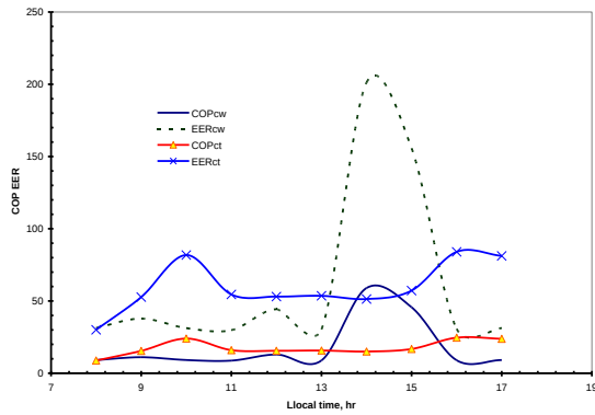
Fig. 8.0 Plot of COP, EER of Cooling Water Tower And Cooling Water against Local Time
