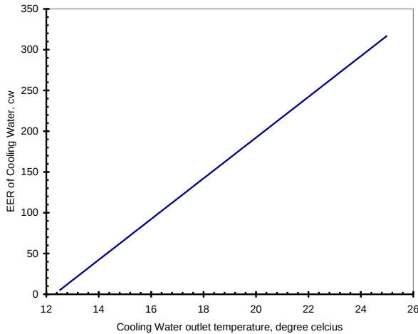
Fig. 4.0 Plot of EER of Cooling Water against Cooling Water Outlet Temperature
