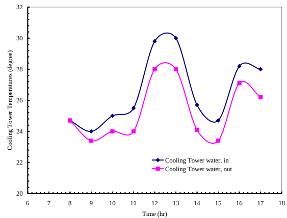
Fig. 11.0 Plot of Cooling Tower Water Entry and Exit Temperatures against Local Time
