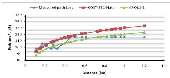
Figure 8: The path Loss (dBm) variation against distance (km) for BTS 5 at Offa Rd., Ilorin, Nigeria
