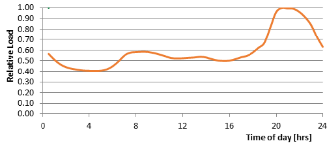
Figure 2: Weekdays load profile.
