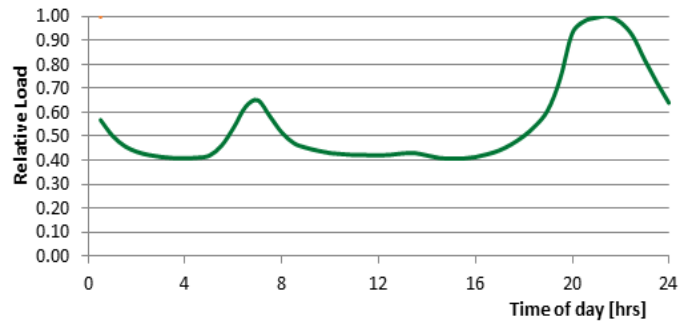
Figure 2: Weekdays load profile.
