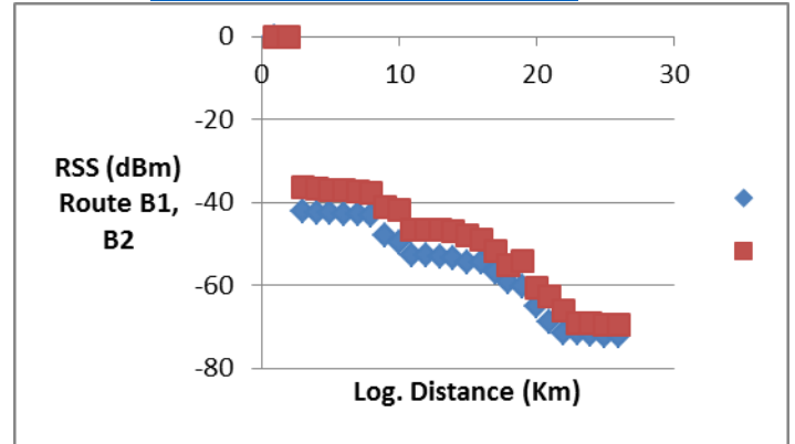
Figure 5 Plot of RSS vs. Log. Distance in Route B 1 , B 2
