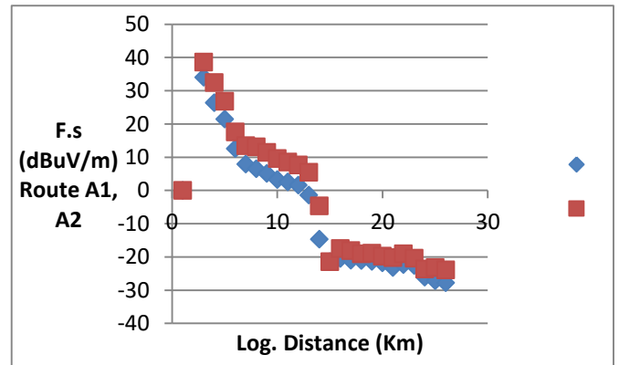
Figure 6 Plot of FS vs. Log. Distance in Route A 1 ,A 2
