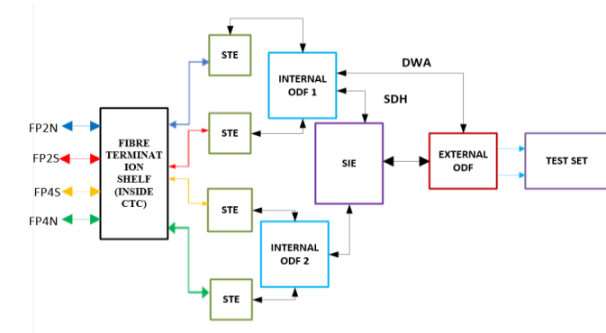
Figure 2: Four -fiber pair submarine system.
