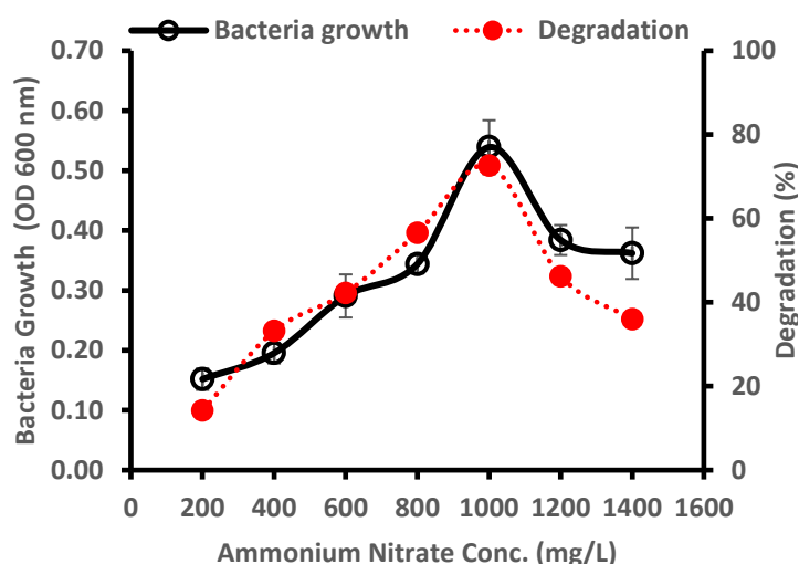
Figure 2. Effect of Ammonium nitrate concentration on the growth and degradation naphthalene by P.stutzeri incubated for 72 h at 37 °C in BH media. Error bars represent mean \pm standard deviation, n=3
