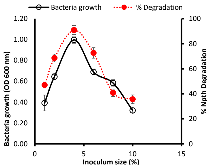
Figure 4: Effect of inoculum size on the growth and degradation of naphthalene by P. stutzeri incubated for 72 h at 37 °C in BH broth. Error bars represent mean ± standard deviation, n = 3
