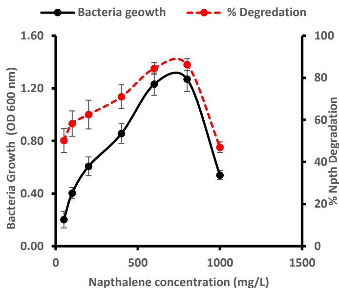
Figure 5: The effect of substrate (naphthalene) concentration on the growth and degradation by P. stutzeri incubated for 72 h at 37 °C in BH media. Error bars represent mean ± standard deviation, n = 3
