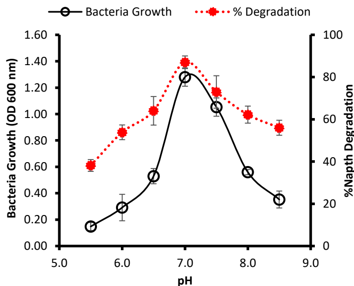
Figure 3. The effect of initial pH on the growth and degradation naphthalene by P.stutzeri incubated for 72 h at 37 °C in BH media. Error bars represent mean \pm standard deviation, n=3
