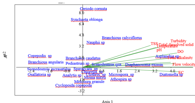
Figure 2. Triplot of first and second Canonical correspondence analysis of plankton and physicochemical characteristics of Bosso Dam and Fadipe Pool Minna Niger state.
