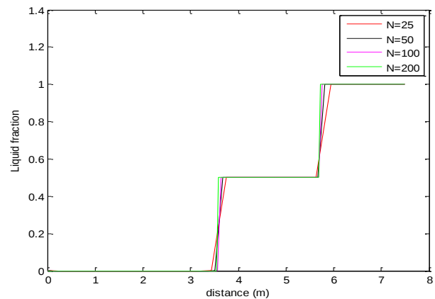
Figure 10 Mesh refinement for the liquid fraction at time t=0.6s using Steger Warming flux vector splitting scheme
