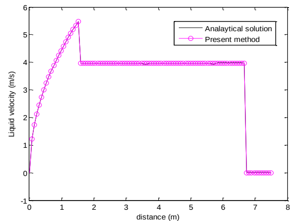
Figure 4 Analytical solution for liquid velocity at t=0.6 \text{ s} and 100 cells compared to the Steger Warming flux vector splitting scheme
