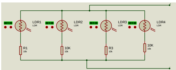
Figure I: The Sensing Circuit
