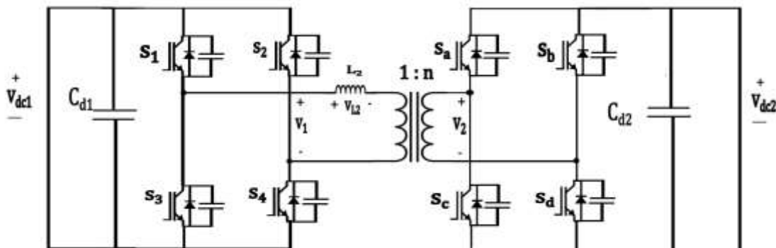
Figure 4: Dual Active Bridge Converter.
