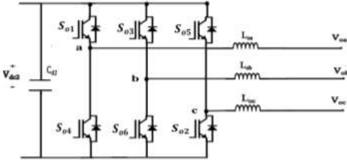
Figure 5: Output Inverter.
