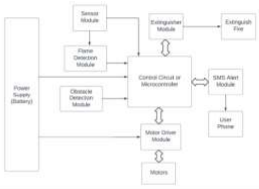
Figure 3 System Design of the Fire Sensing and Extinguishing Robot.
