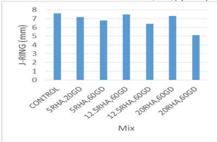
Figure 3: Result of J-ring test.
