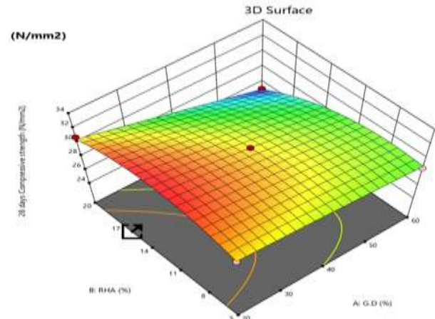
Figure 6: 3D response surface for 28-day compressive strength
