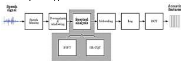
Figure 5: How Spectral analysis is applied in speech signal processing [27].
