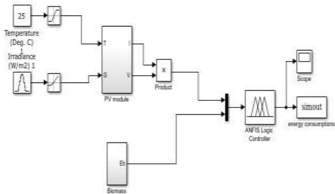
Figure 14: Complete system modeling
