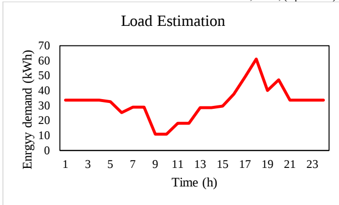
Figure 8: Kebisoni community load estimation
