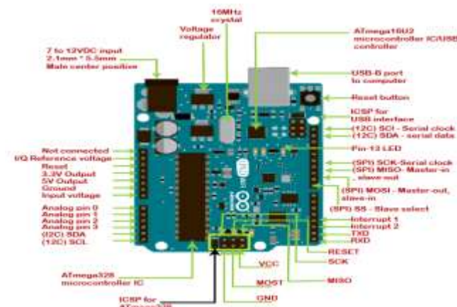
Figure 2 Arduino Uno pin configuration
