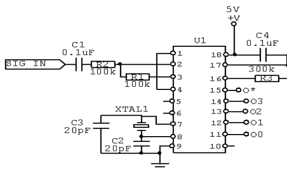
Figure 3: Circuit Diagram of HT 8870 DTMF Decoder
