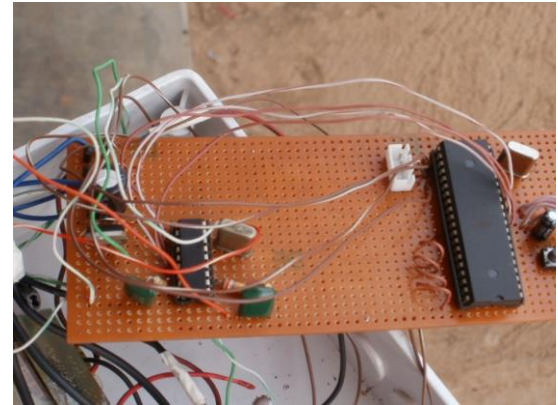
Figure 7: Microcontroller with other Components on Construction Board
