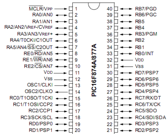
Figure 2: Pin configuration of PIC 16F877A (Micro-Controller)
