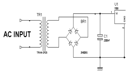
Figure 6: Rectifier Circuit
