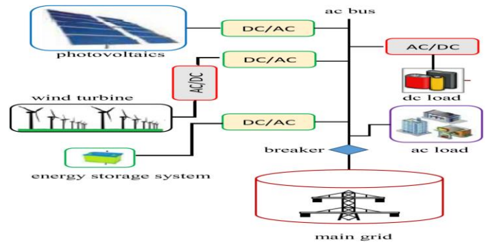
Figure 6: AC microgrid configuration [24]
