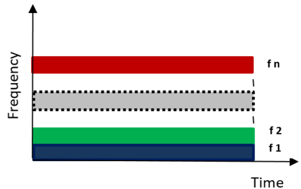
Figure 2.1: Frequency Division Multiplexed signal for satellite Application.
