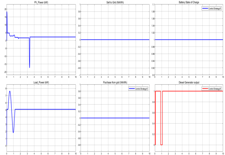
Figure 7: Islanding mode
